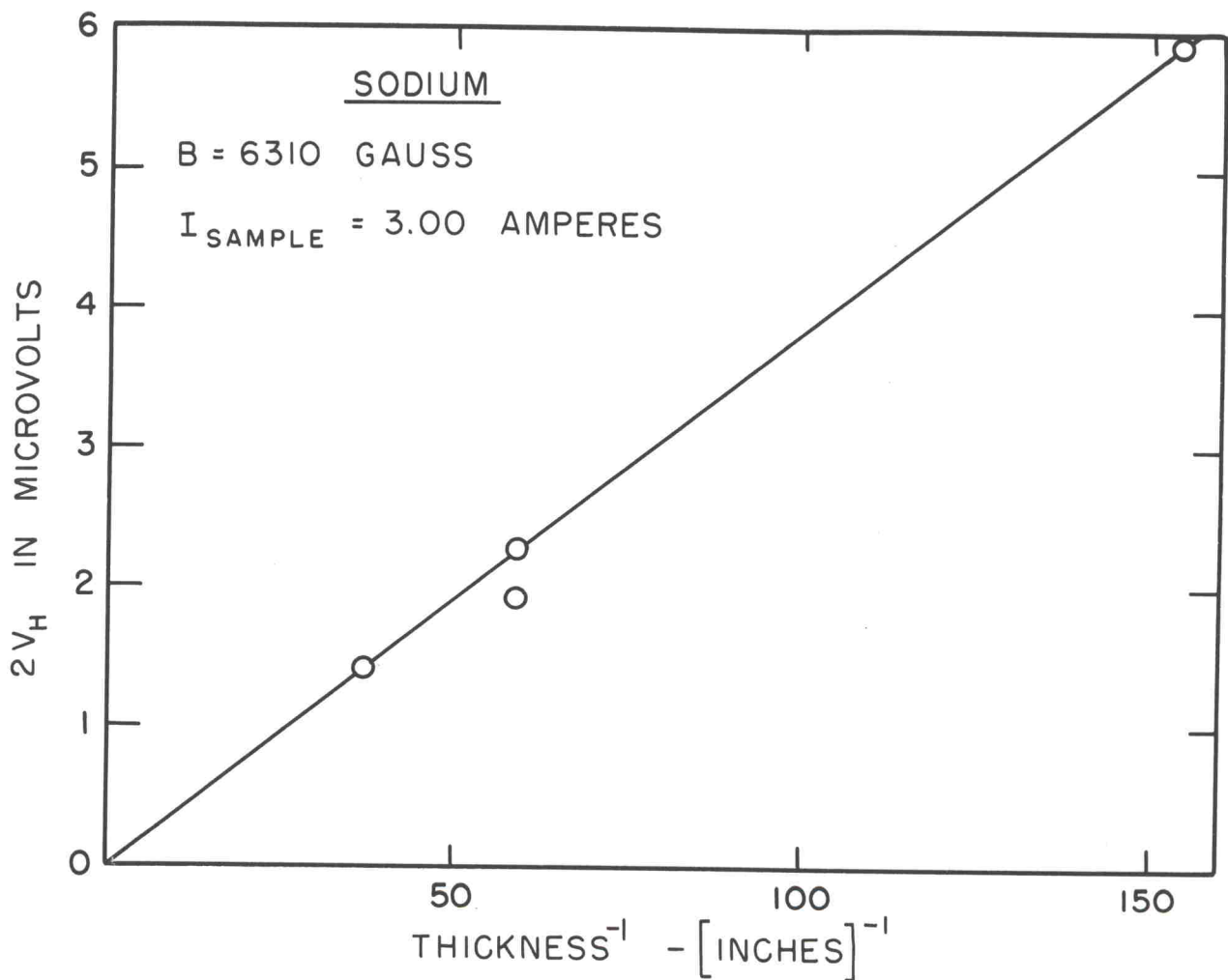
FIG. 3-17 HALL VOLTAGE \times 2 , 2V_H , VS. SAMPLE THICKNESS -1
